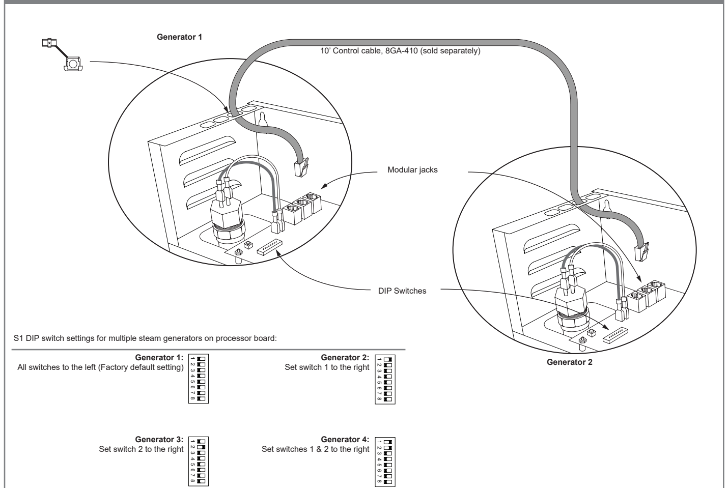
Figure 3 - Ganging Steam Generators (when applicable)
