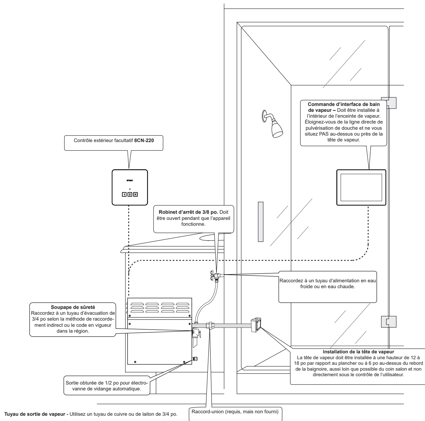
Figure 3 - Installation typique
