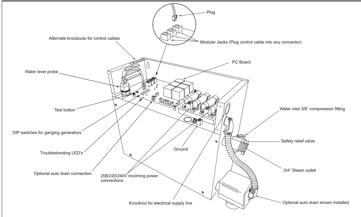
Figure 2 - Internal Electrical Connection
