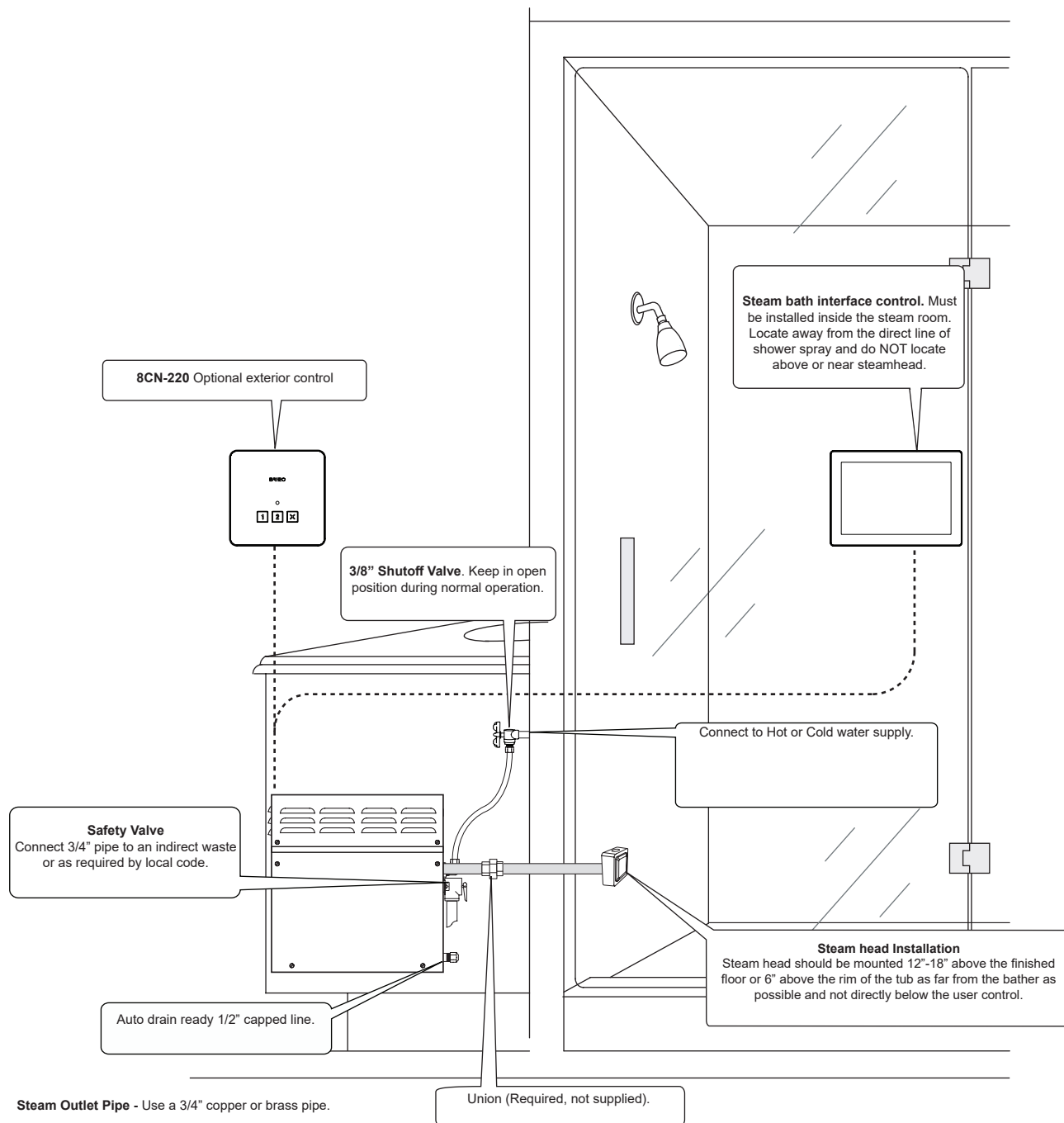
Figure 3 - Typical Installation
