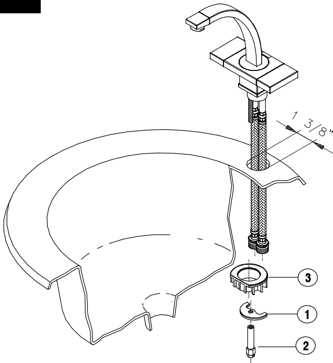
Fig. 1. FAUCET INSTALLATION
