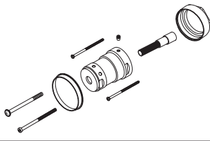
RP47201 Cartridge Assembly Cartucho Cartouche
