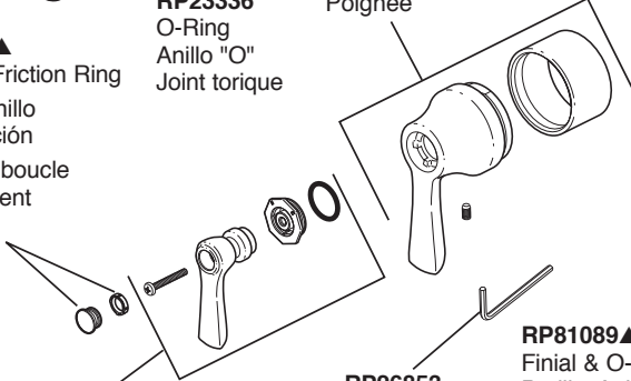
RP26853 Allen Wrench Llave Clé
